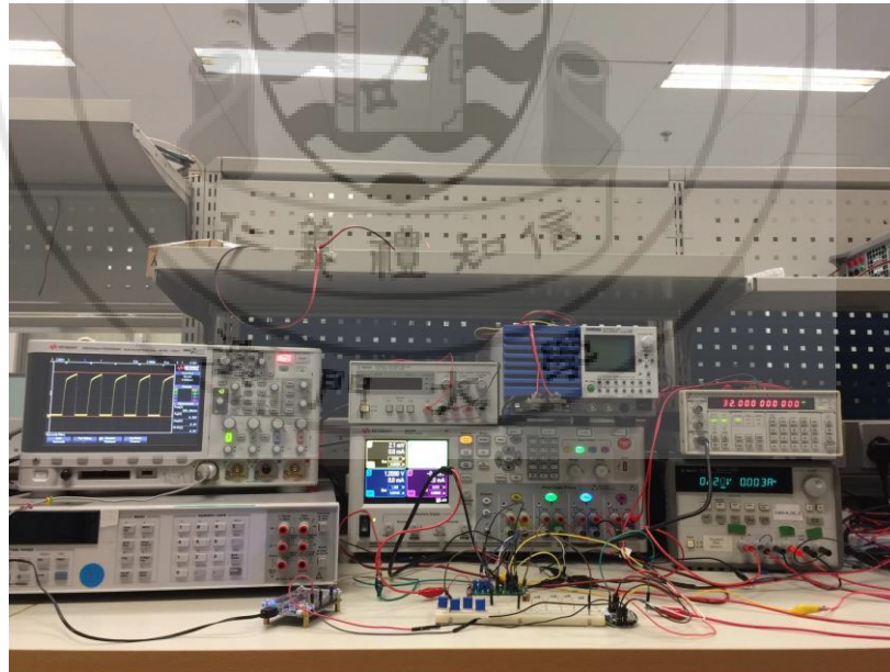
Figure 23 Measurement setup of the chip prototype
