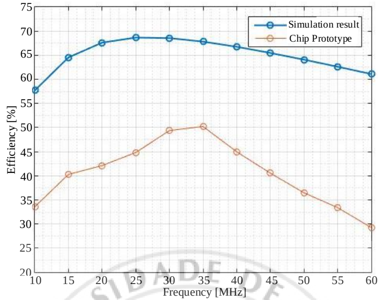
Figure 25 The comparison of the simulation and chip measurement results
