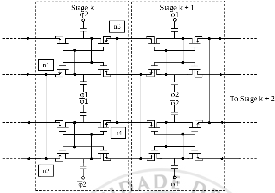
Figure 4 Proposed driver architecture of two successive driver stage in [1]
