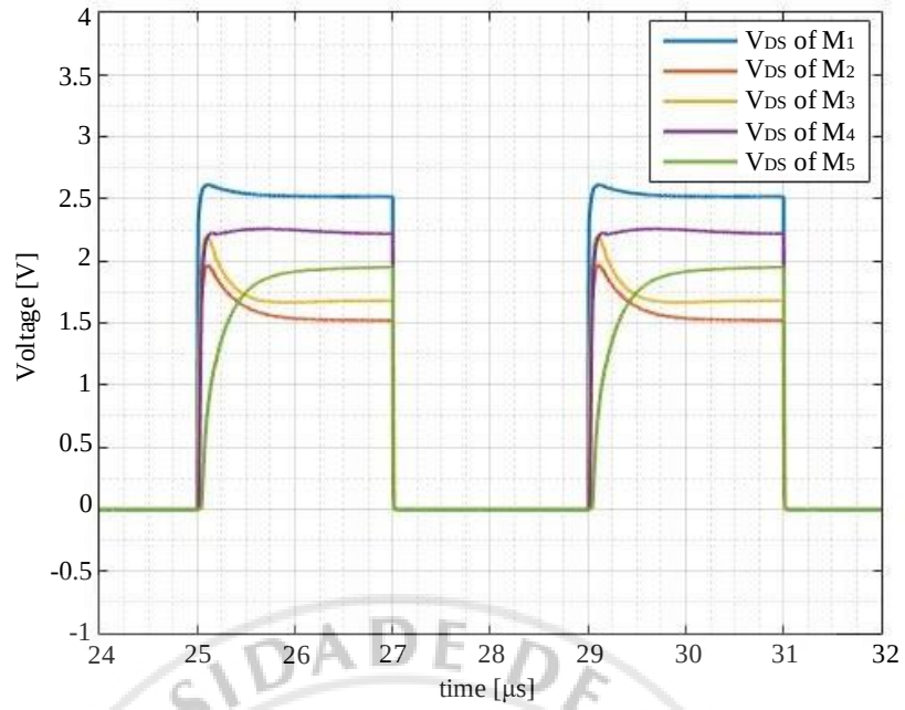
Figure 17 V_{DS} of stacked output transistors of the n-switch block without low-pass filter
