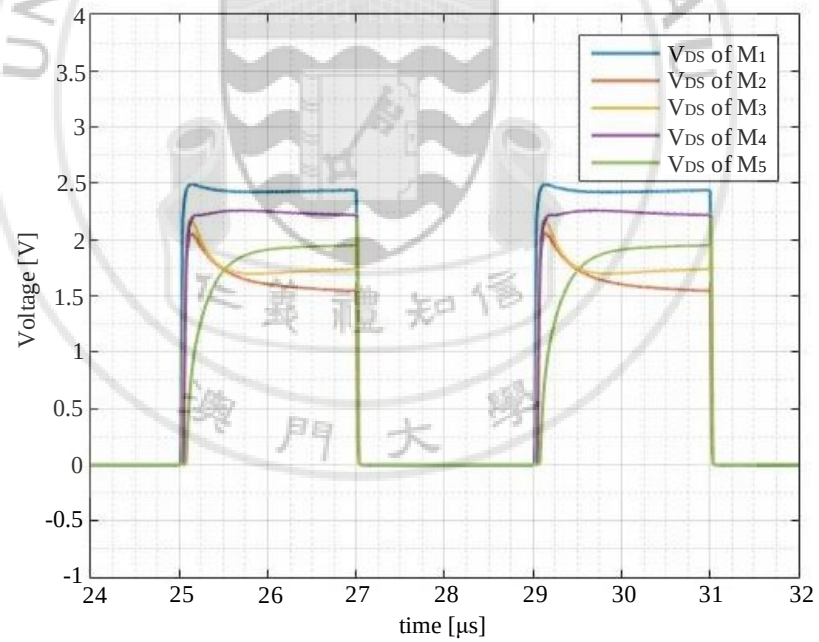
Figure 18 V_{DS} of stacked output transistors of the n-switch block with low-pass filter
