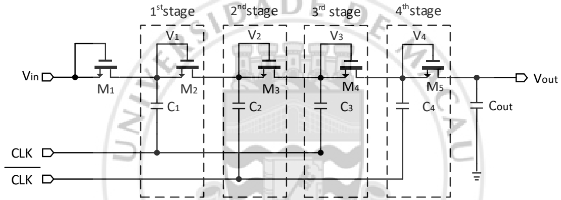
Figure 3 The modified Dickson Charge Pump by placing NMOS transistor instead of diode
