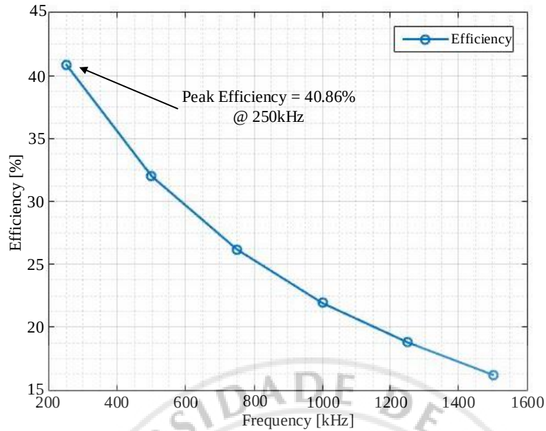
Figure 24 The efficiency of the MEMS Drivers
