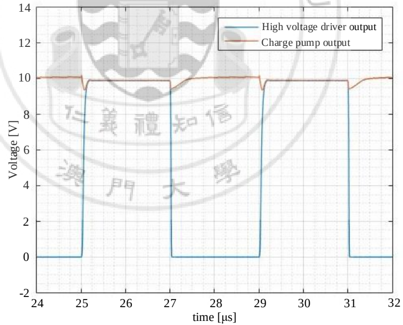
Figure 13 The outputs of the circuit
