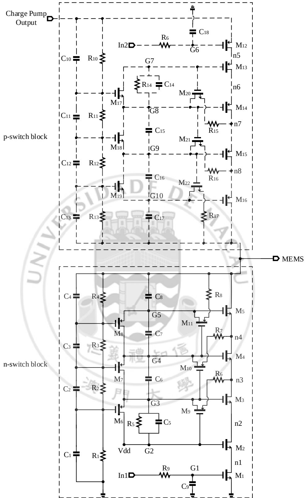
Figure 12 The schematic of the proposed high voltage driver
