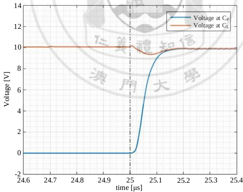
Figure 21 The outputs with compensation capacitor C_C
