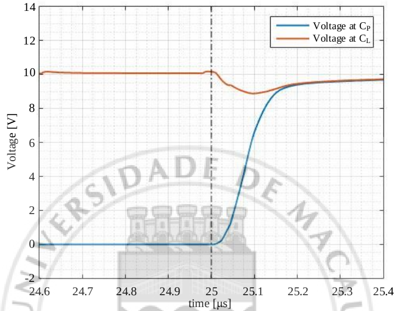
Figure 19 The illustration of the charge sharing
