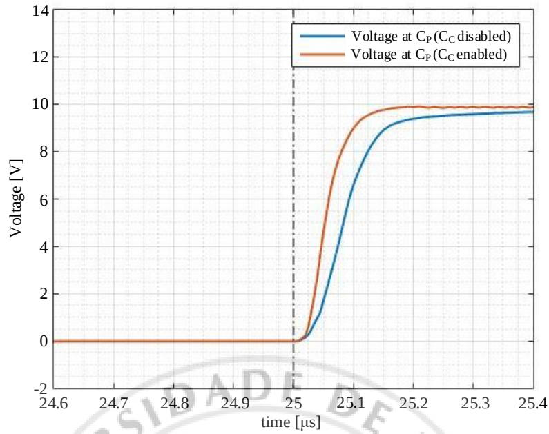
Figure 22 The driver outputs under the appearance of C_C
