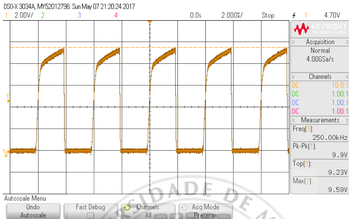
Figure 26 Measurement result of chip prototype
