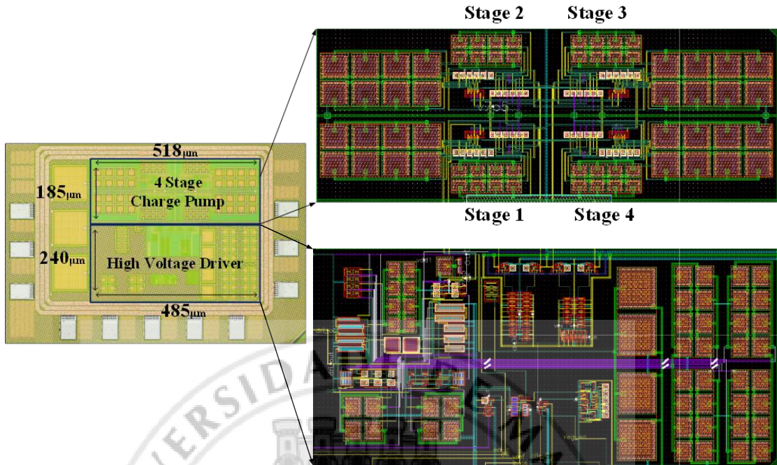
Figure 14 Micrograph of the 65nm CMOS die with all 4 sub-pumps and high voltage Driver high-lighted
