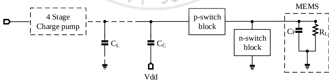
Figure 20 The schematic of the circuit with charge sharing compensation capacitor C_c
