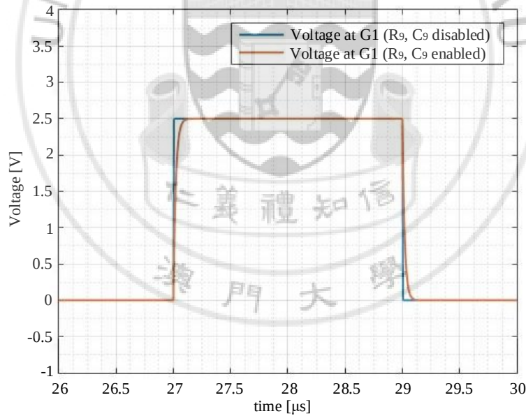
Figure 16 The voltage at node G1 under different condition
