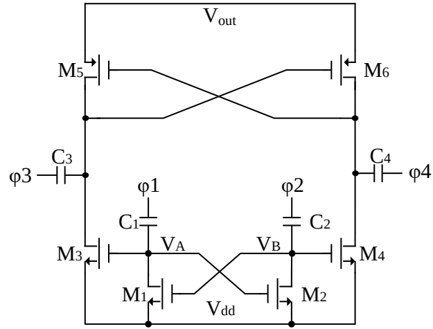
Figure 7 The proposed architecture of the charge pump
