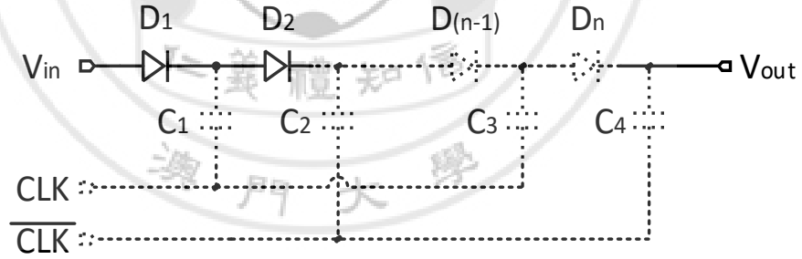
Figure 2 Schematic of Diode based Dickson Charge Pump
