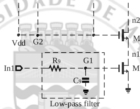
Figure 15 The low-pass filter ( R_9 , C_9 ) embedded at the gate of M_1 of n-switch block
