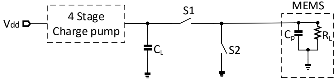
Figure 6 The block diagram of this work
