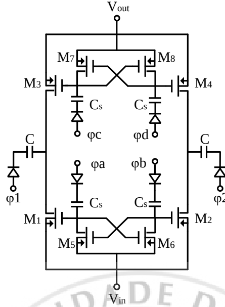
Figure 5 One stage of the proposed architecture in [7]
